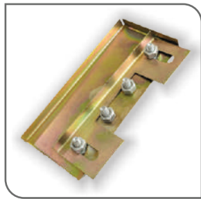
Magnet Tray
